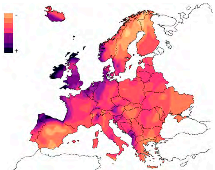
Hazard of decay fungi growth (Scheffer index)
